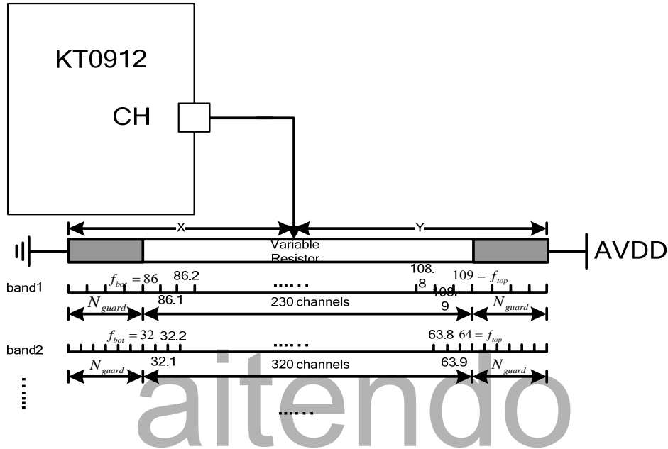
Figure 5: CH pin connection in dial-mode
